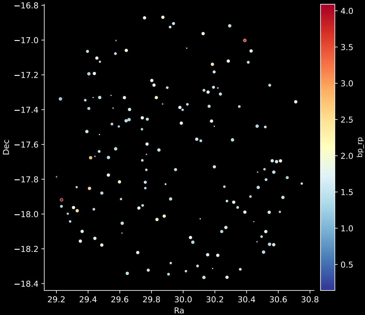
APOGEE DR17 Field: [020-14] Stars: 148
