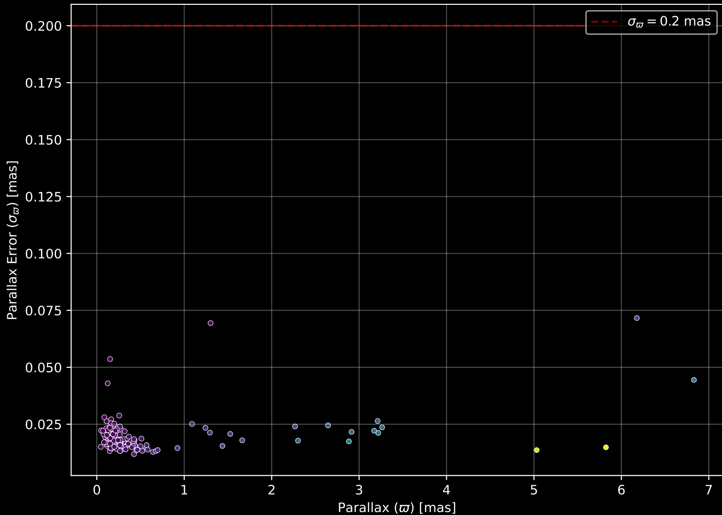
APOGEE DR17 Field: [020-14] Parallax Quality (n= 148)
