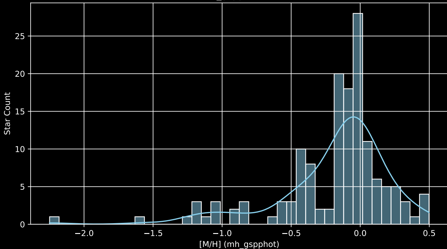
APOGEE DR17 Field: [020-14 [M/H] (mh_gspphot) (n= 145)
