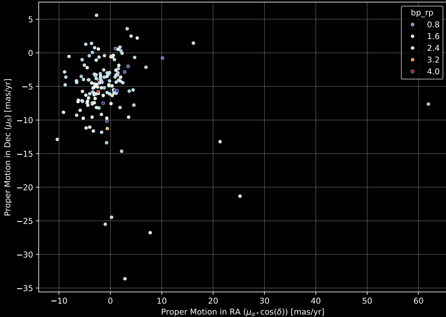
APOGEE DR17 Field: [020-14] Proper Motion Diagram (n= 148)
