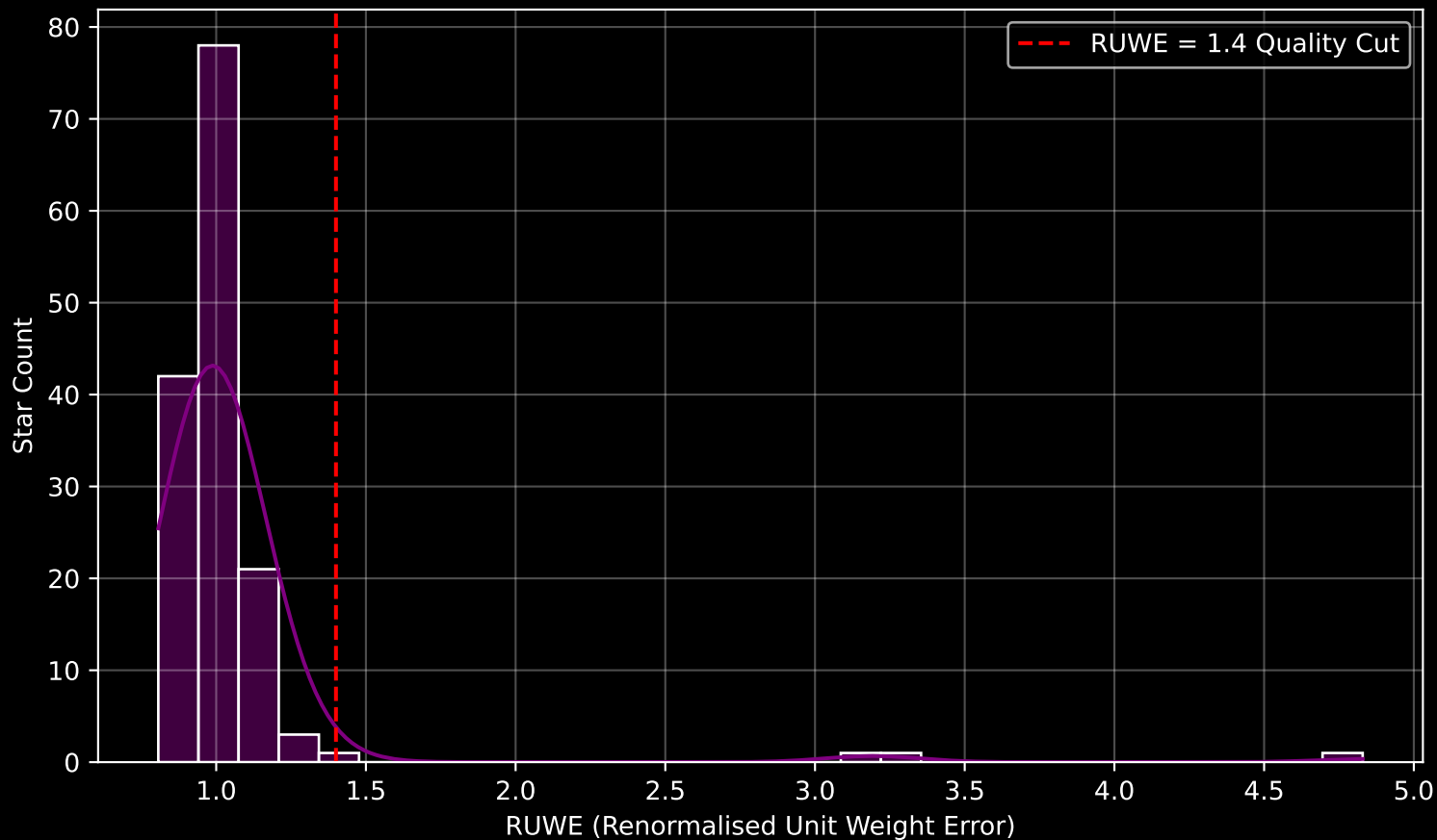
GAPOGEE DR17 Field [020-14] RUWE Distribution (n= 148)
